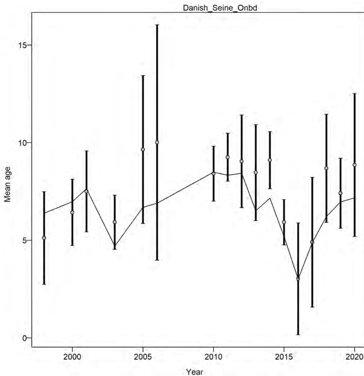
Figure A 8.39. Mean age (aggregated across length bins) for eastern Jackass Morwong from Daish seine with 95% confidence intervals based on current samples sizes. Punt data weighting method TA1.8: Thin capped lines matching thick lines indicate this is well balanced. Yearly variation in the data is shown in changes in mean age, which can be large over a short period.
