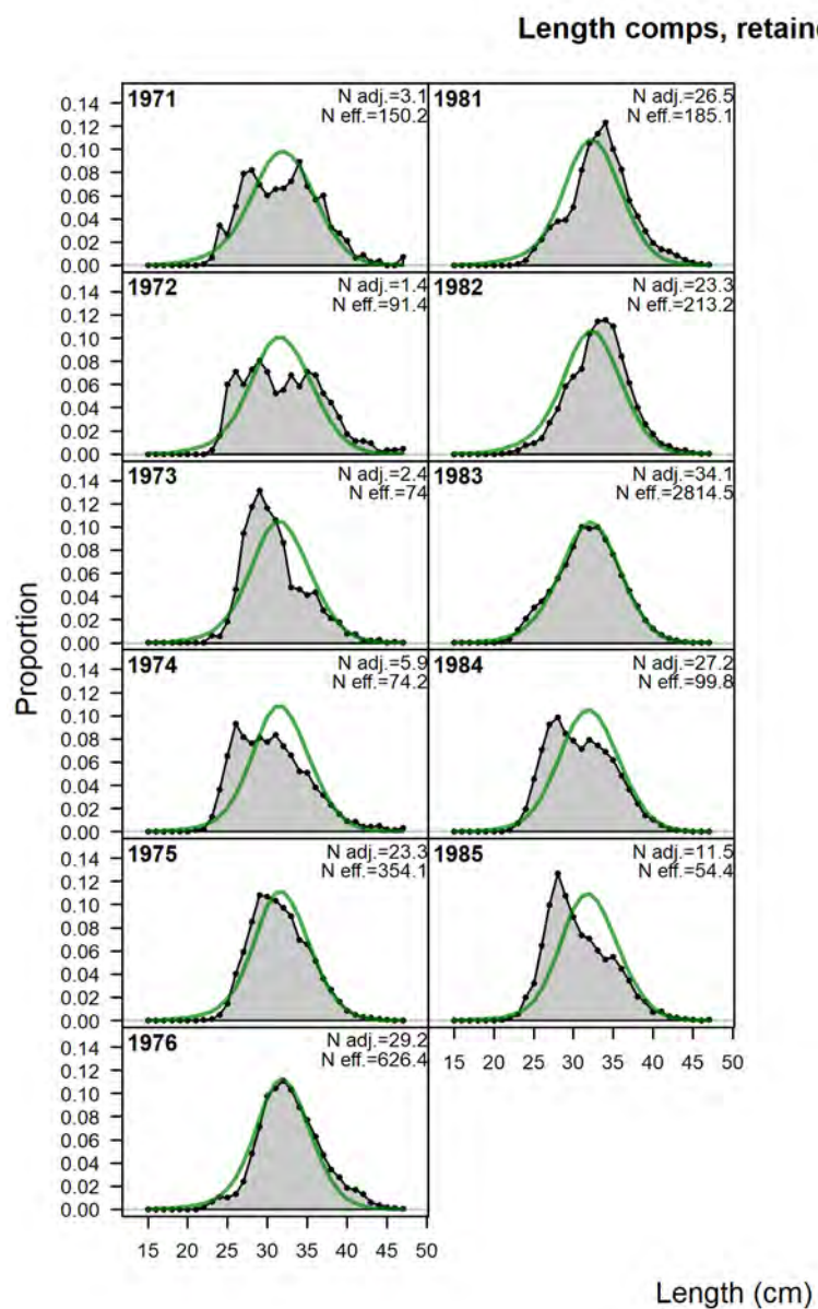
Figure A 8.3. Eastern Jackass Morwong length composition fits: mixed fleet retained.
