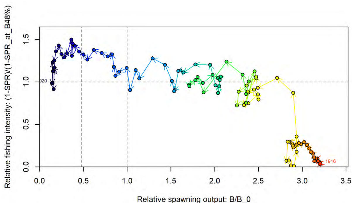
Figure 8.22. Kobe plot for the base case, showing the trajectory of spawning biomass (relative to B_0 ) plotted against 1-SPR, which is a proxy for fishing mortality, essentially integrating fishing mortality across fleets in the fishery. The horizontal line indicates the target fishing intensity that should theoretically result in the population reaching B_{48} .
