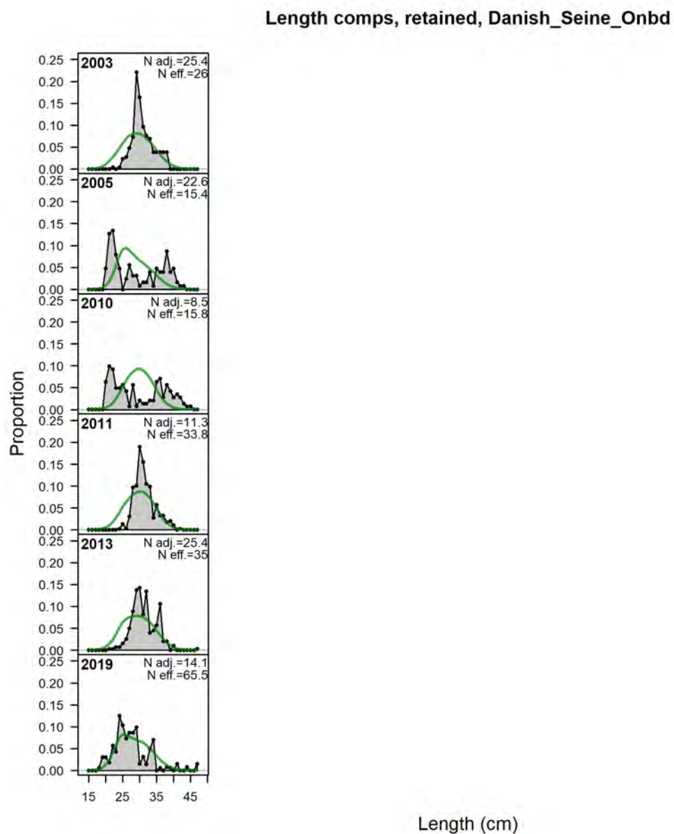
Figure A 7.23. Eastern Jackass Morwong length composition fits: Danish seine onboard retained.
