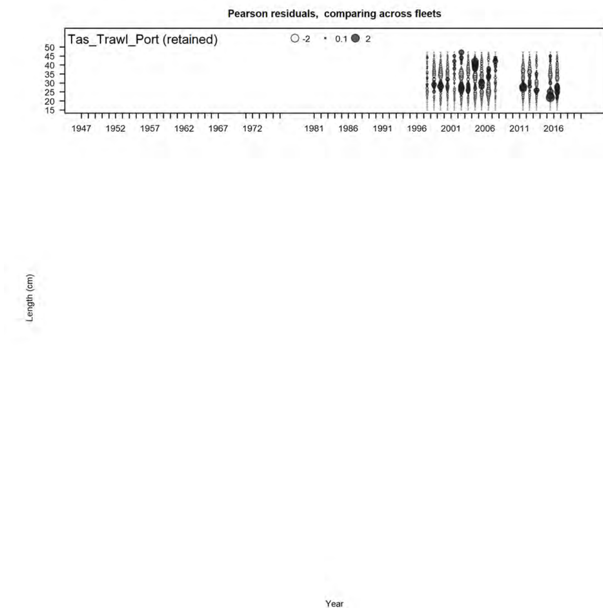
Figure A 8.17. Residuals from the annual length composition data for eastern Jackass Morwong displayed by year and fleet Tasmanian trawl fleet (retained port).
