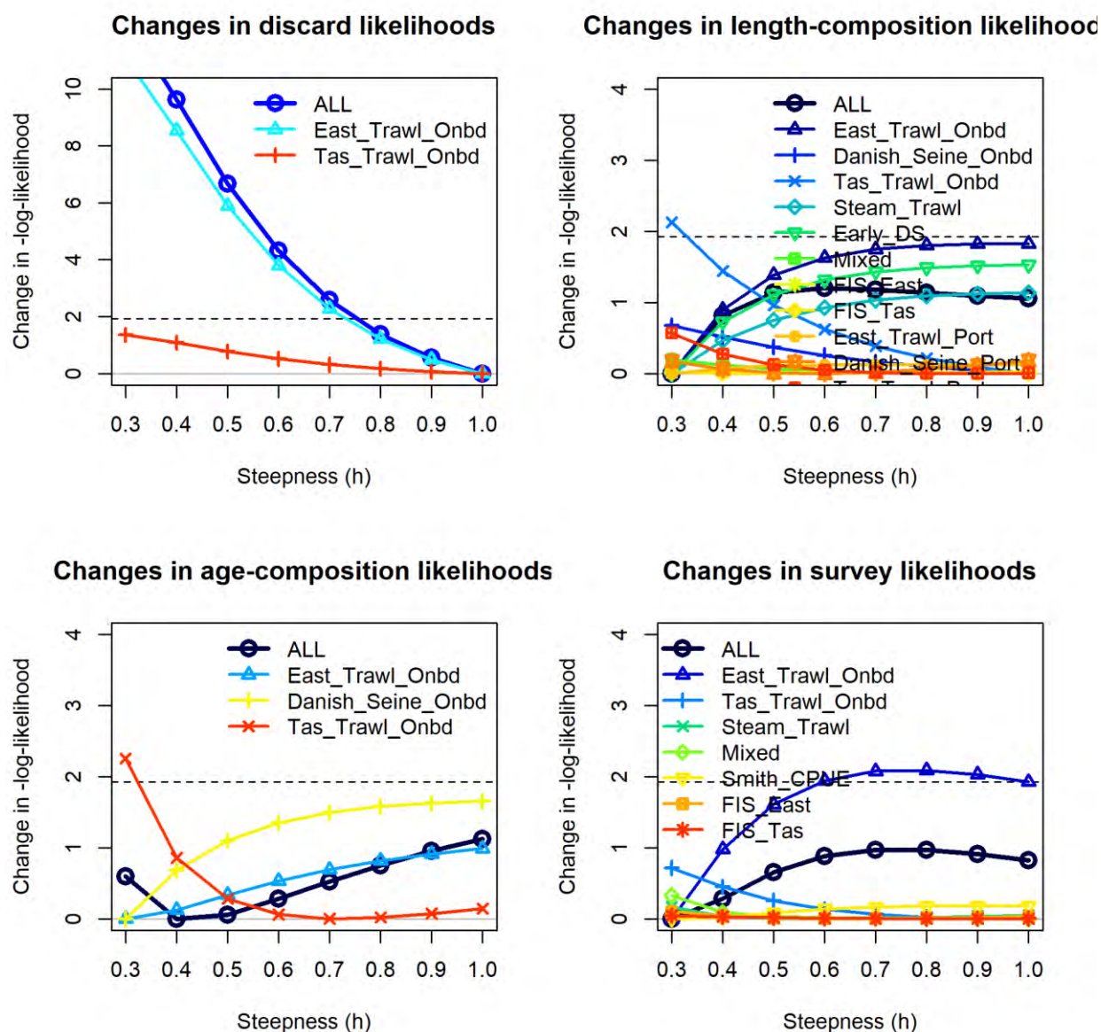
Figure 8.44. Piner plot for the likelihood profile for steepness for the base case with low recruitment, showing components of the change in likelihood for discard rate estimates, length, age, and surveys (CPUE) by fleet.
