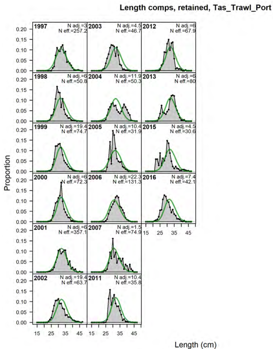
Figure A 7.26. Eastern Jackass Morwong length composition fits: Tasmanian trawl port retained.
