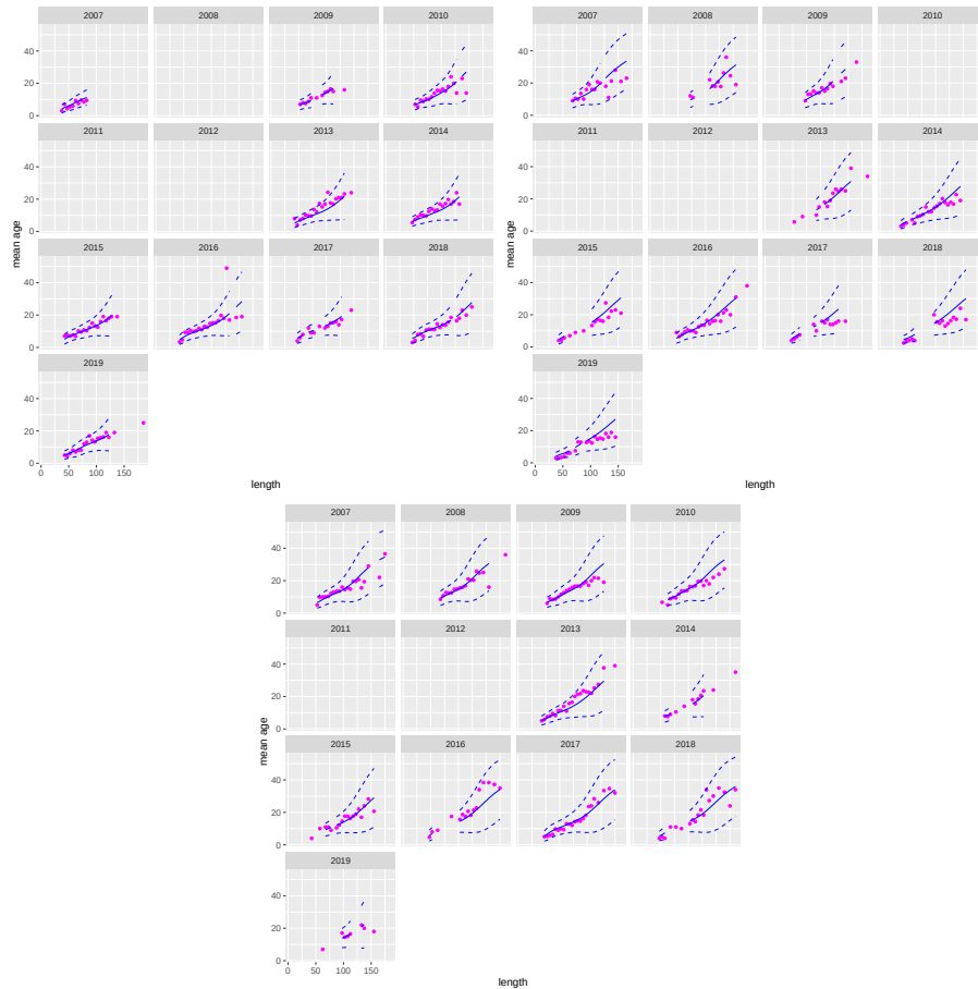
Figure 6.5: Fits to the ATL (top left), NMRL (top right), and SMRL (bottom) longline fisheries female age-given-length data. Magenta circles are the observed mean age, and the blue lines the predicted median and 95%ile.
