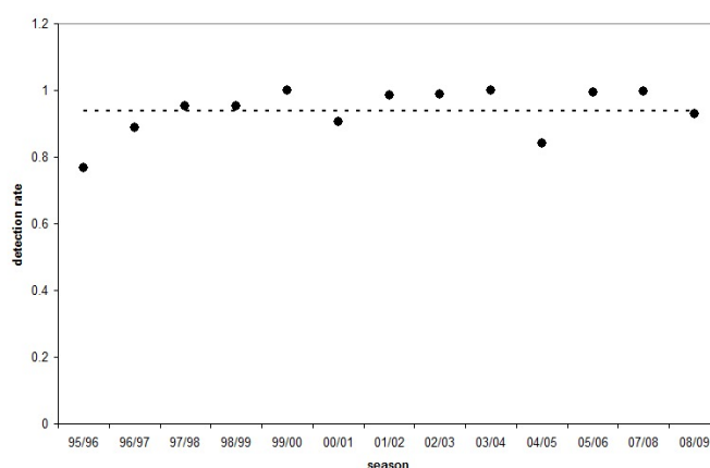
Figure 3.2: Estimated tag detection rate (points) by fishing season [7]. Dotted line corresponds to the mean detection rate (0.938) over the time series.
