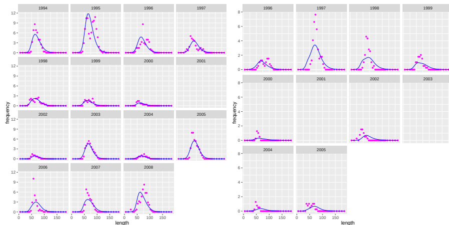
Figure 6.1: Fits to the ATT (left) and NVT (right) trawl fisheries length data. Magenta circles are the observed data, and the blue lines the predictions.
