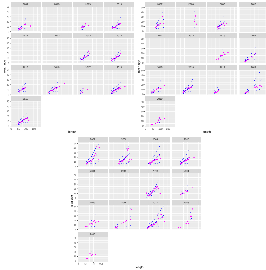
Figure 6.6: Fits to the ATL (top left), NMRL (top right), and SMRL (bottom) longline fisheries male age-given-length data. Magenta circles are the observed mean age, and the blue lines the predicted median and 95%ile.
