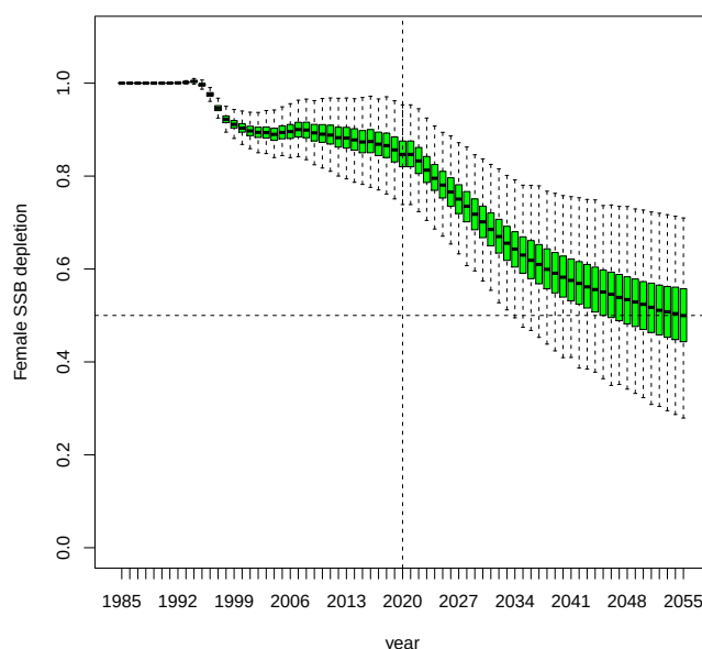
Figure 7.1: Projection for one of the recommended TAC scenarios in Table 7.1.
