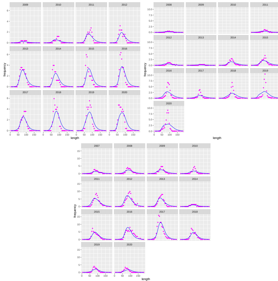
Figure 6.2: Fits to the ATL (top left), NMRL (top right), and SMRL (bottom) longline fisheries length data. Magenta circles are the observed data, and the blue lines the predictions.
