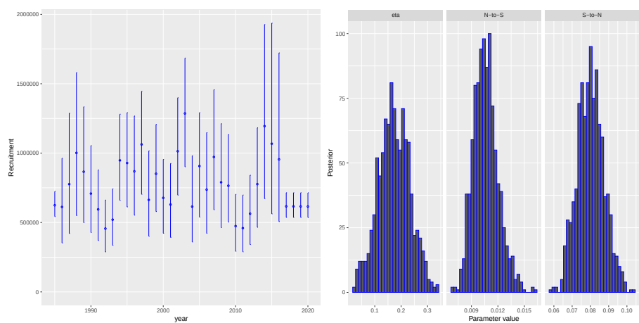
Figure 6.9: Posterior median and 95% credible intervals for total recruitment (left), and the marginal posteriors for the three spatial parameters: \eta_1 , \Phi_{1,2} , and \Phi_{2,1} (right).
