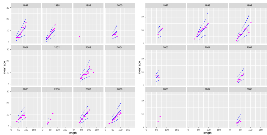
Figure 6.4: Fits to the ATT (left) and NVT (right) trawl fisheries male age-given-length data. Magenta circles are the observed mean age, and the blue lines the predicted median and 95%ile.
