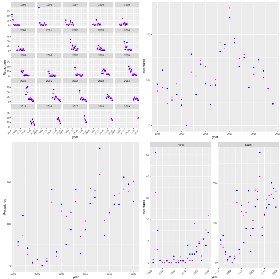
Figure 6.7: Fits to the tagging data (blue circles, observed; magenta triangles, predicted) for recaptures following year of release (top left), total recaptures for each year of release (top right), total recaptures for year of recapture (bottom left), and recaptures for each year and region of recapture (bottom right).
