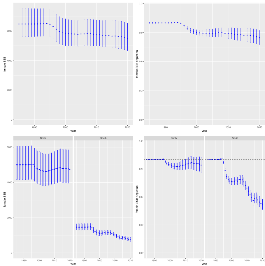
Figure 6.8: Posterior median and 95% credible intervals for total female SSB (top left), female SSB relative depletion (top right), spatial female SSB (bottom left), and spatial female SSB relative depletion (bottom right).
