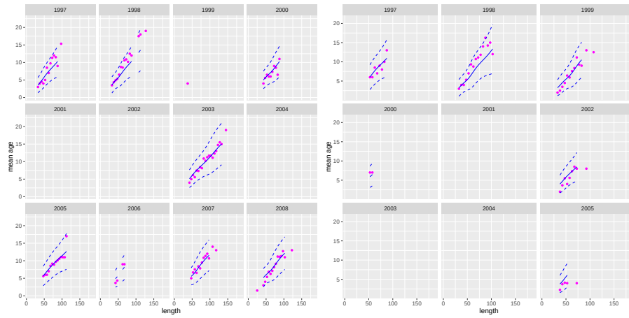
Figure 6.3: Fits to the ATT (left) and NVT (right) trawl fisheries female age-given-length data. Magenta circles are the observed mean age, and the blue lines the predicted median and 95%ile.
